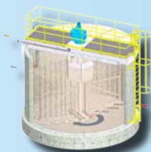
Thickner
